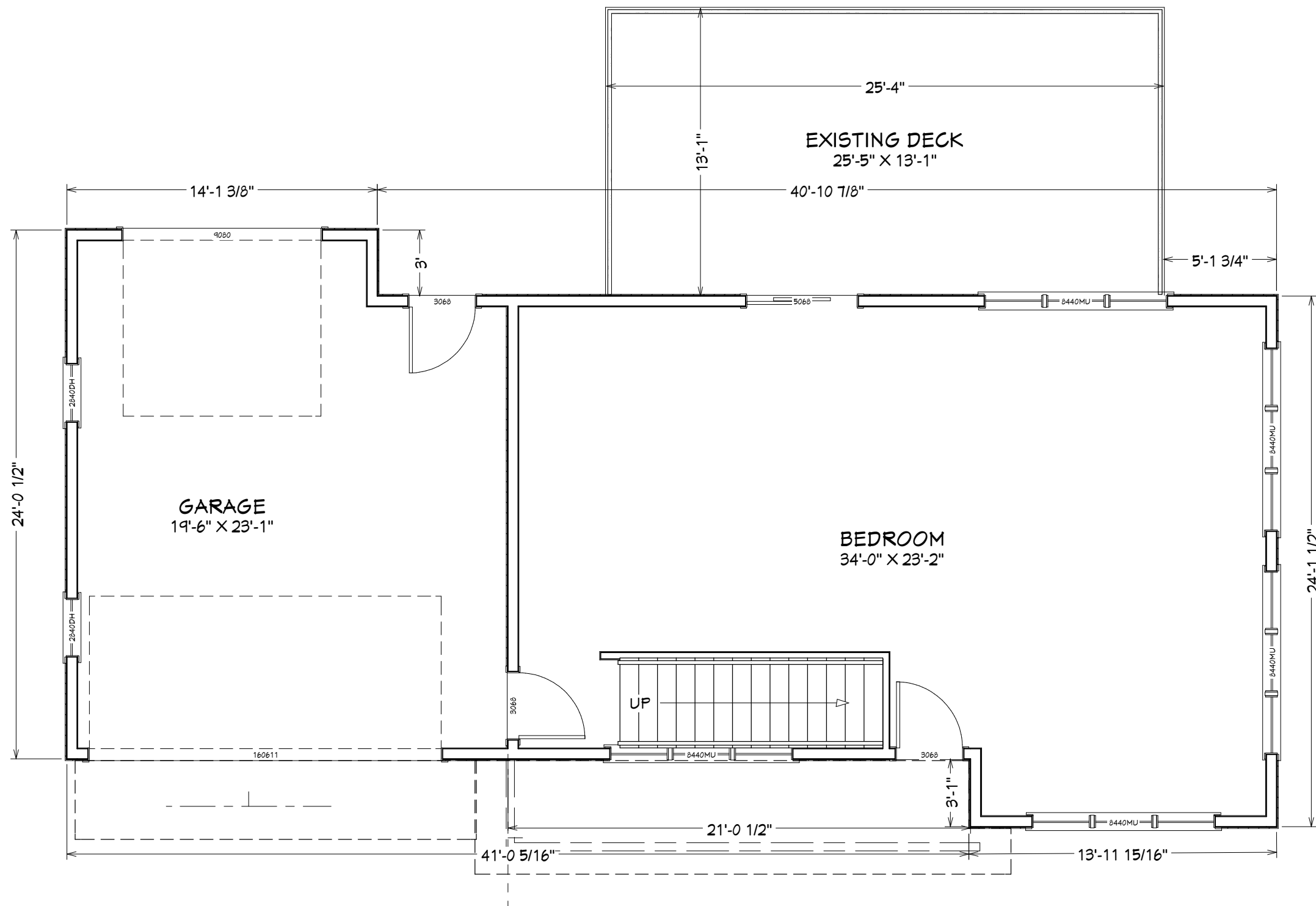
FIRST FLOOR AND EXISTING DECK
