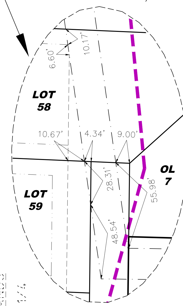
DETAIL NO SCALE
