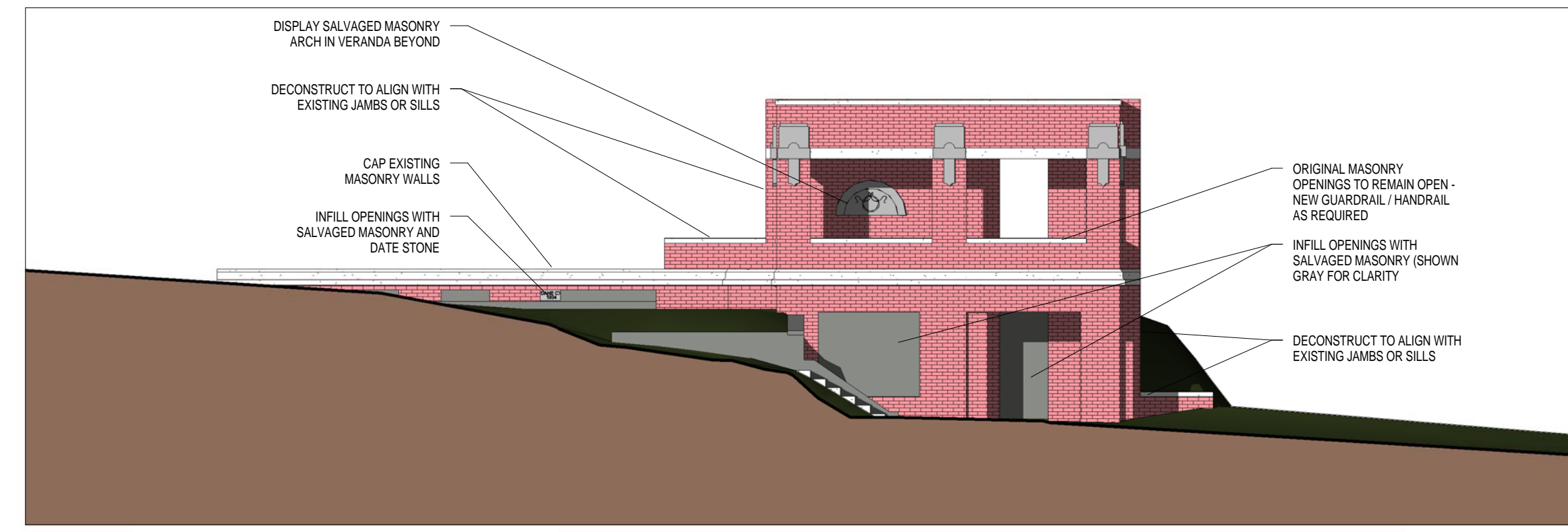
WEST ELEVATION
