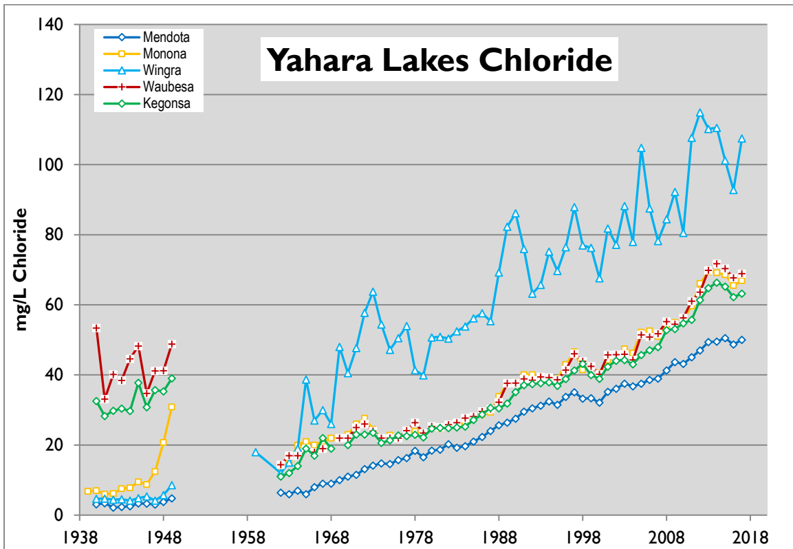
Figure 2: Chloride trends in the Yahara Lakes.
