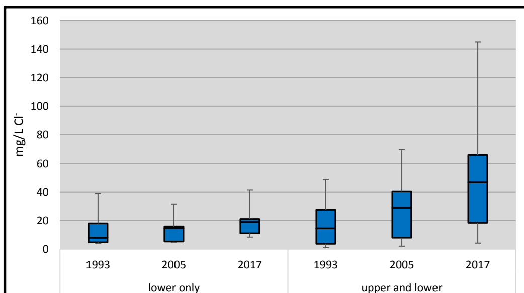
Figure 3: 25-year chloride trend in Madison drinking water.
