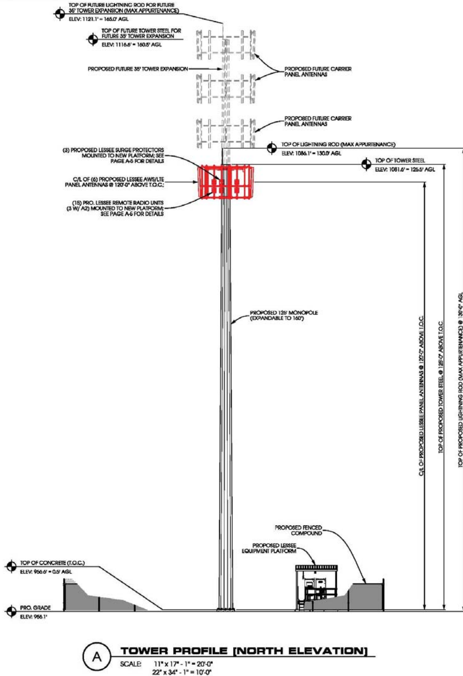
Figure 5 – Vertical Elevation Tower Drawing
