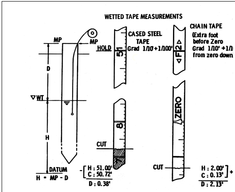
Figure 1. Steel tape.
