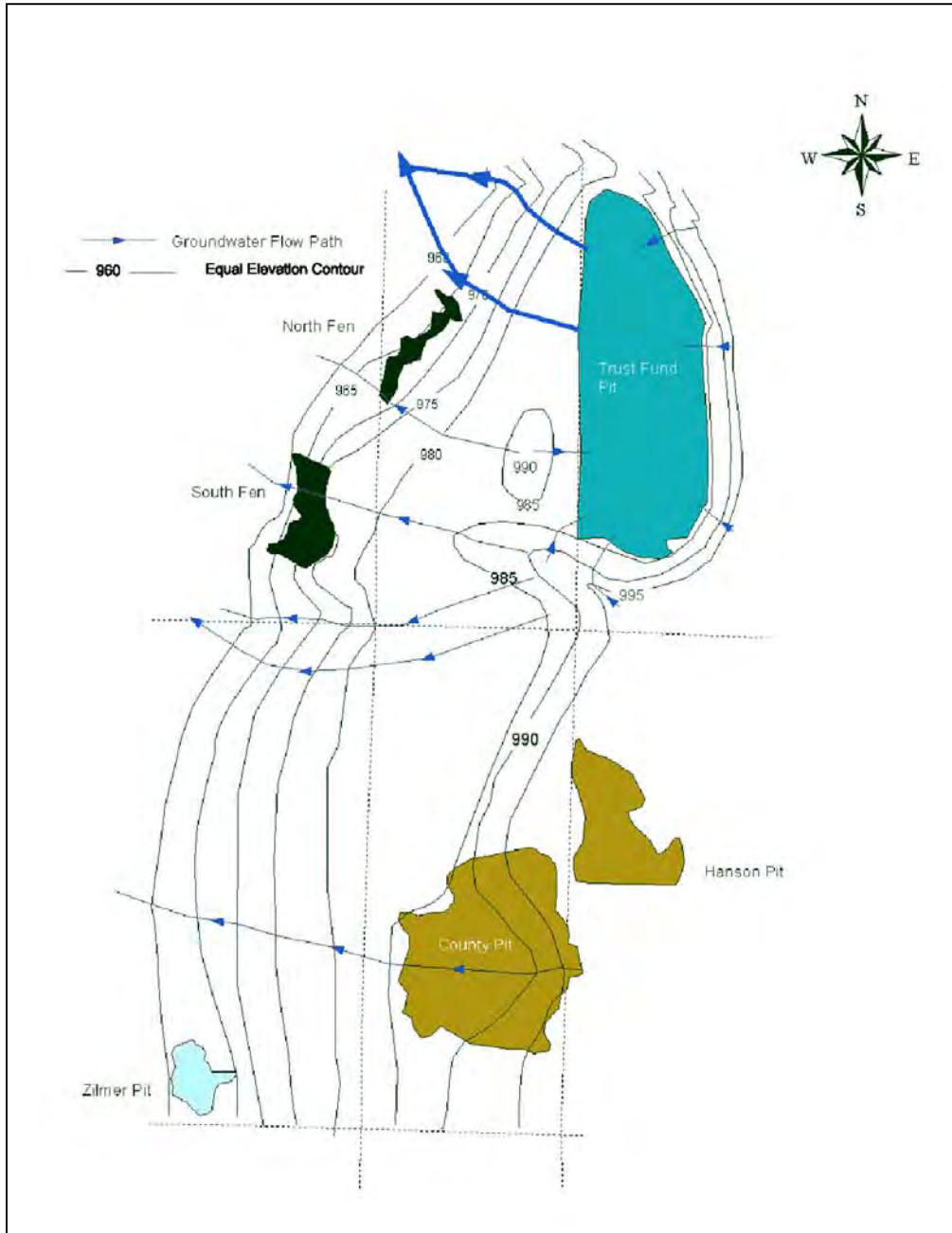
Figure 10.6. Ground-water flow paths (blue) during mining.
