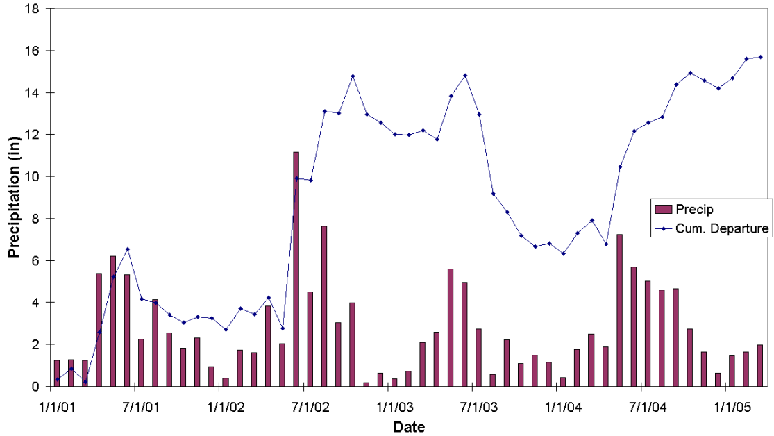
Precipitation Station 217009 with Cumulative Departure from Normal
